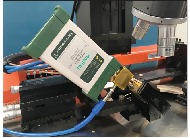
Figure 5. Spectrum Master MS2760A spectrum analyzer enables the test ports
