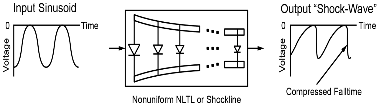
Figure 1. The falling edge of an electrical wave undergoes compression as the wave propagates along the nonlinear transmission line. This effect is analogous to that of a water wave before breaking on the shore.
